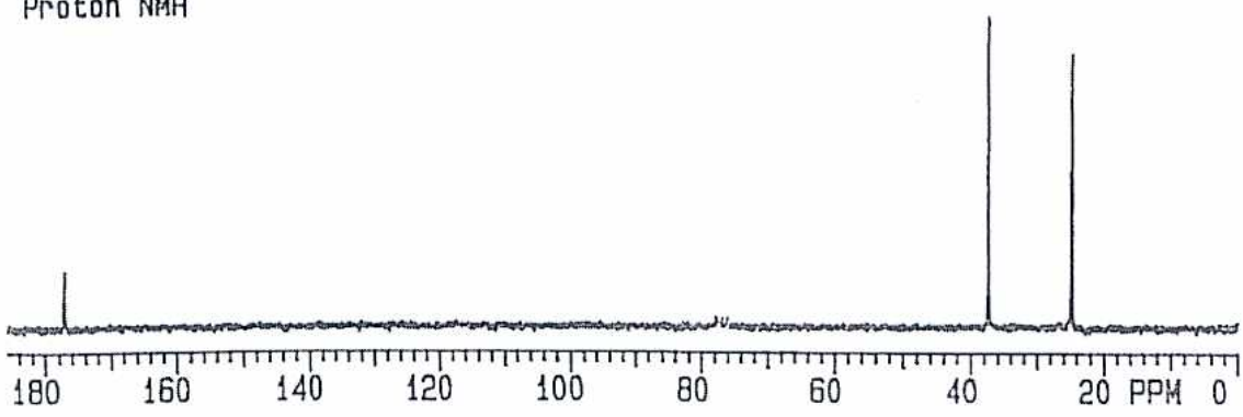
Carbon 13 NMR
