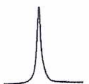
11.6 PPM Proton NMR
